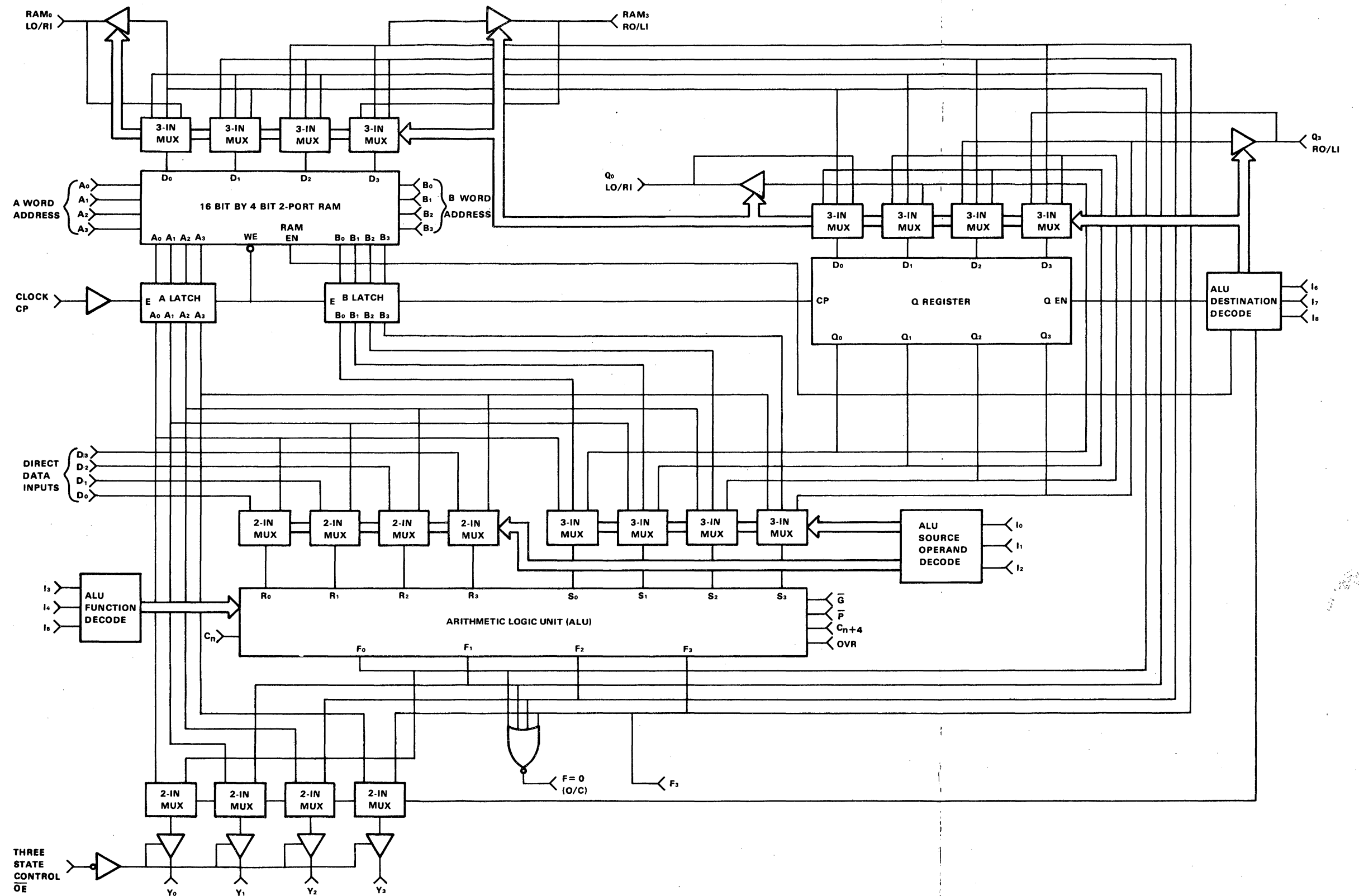
Figure 6-3 Microprocessor (AM2901) Block Diagram
