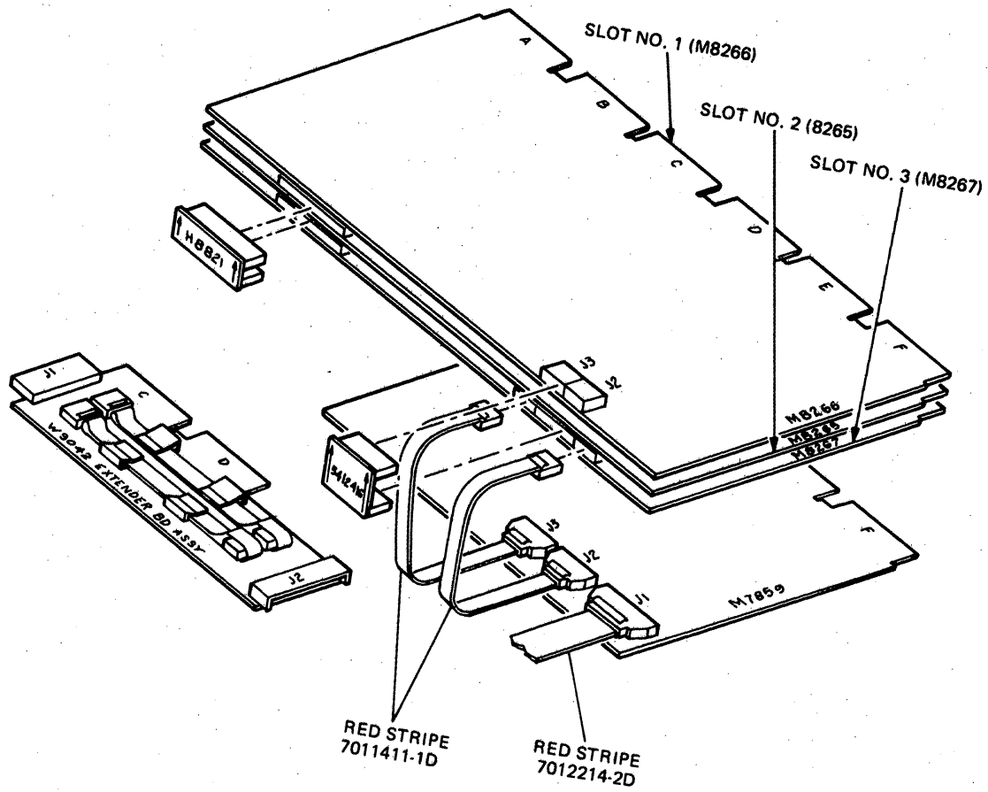
Figure 2-1 Maintenance Cable Installation
