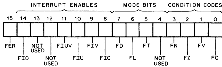
Figure 4-6 FP11-A Status Register Format
