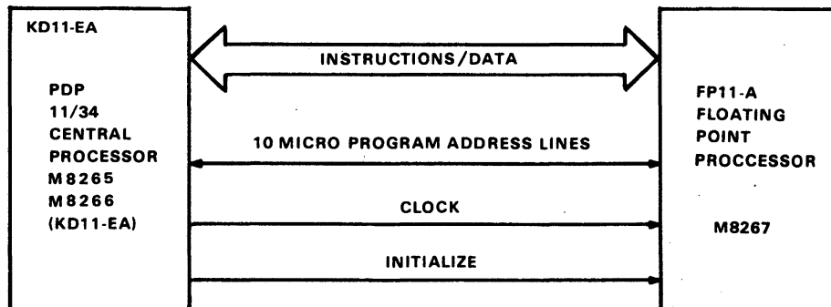
Figure 1-1 KD11-EA/FP11-A Signal Interface
