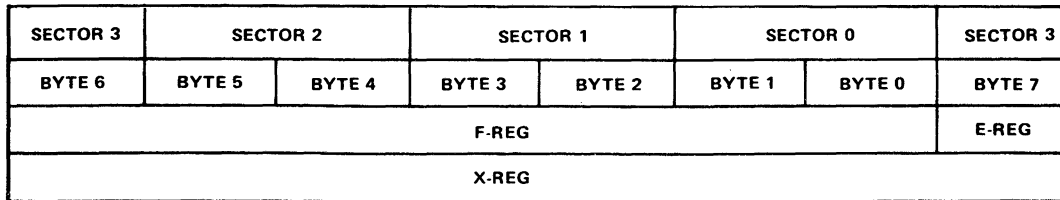
Figure 6-4 RAM Register Usage
