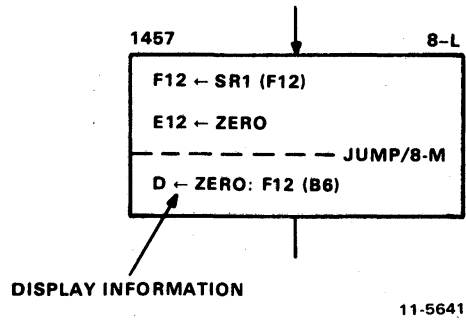
Figure 7-1 Display Information
