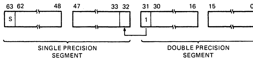
Figure 5-3 Double-to-Single Precision Rounding
