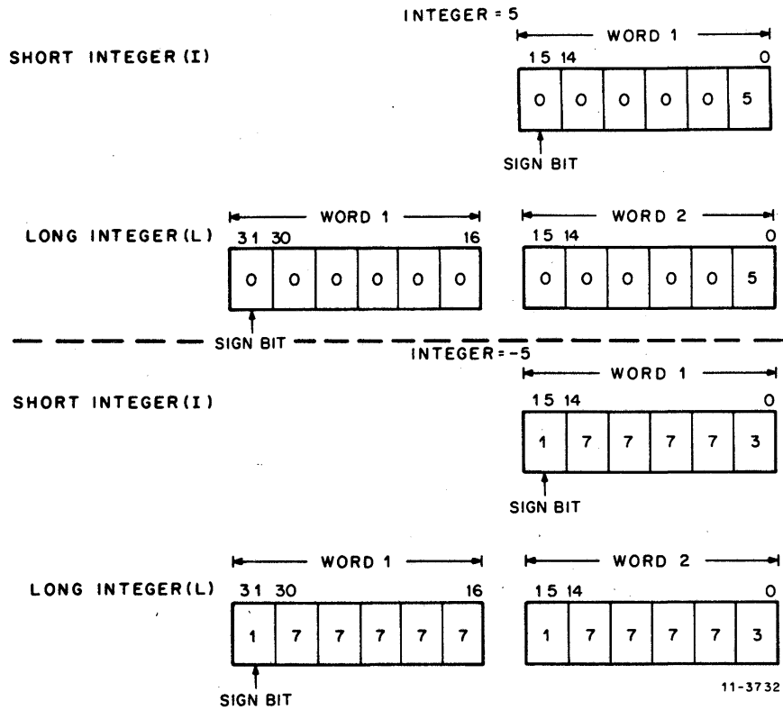
Figure 4-1 Integer Formats
