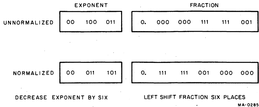
Figure 3-1 Normalization
