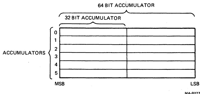
Figure 5-1 Floating-Point Accumulators
