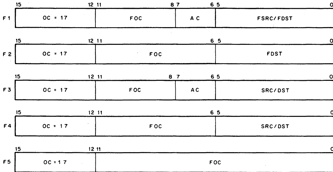
Figure 5-2 Instruction Formats
